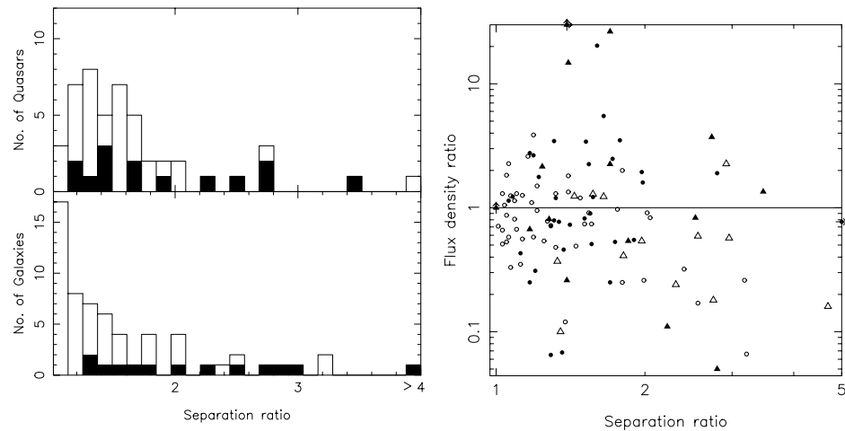
Figure 1 Left: The distributions of the arm-length or separation ratio, r_D , for the sample of high-luminosity FR II radio galaxies and quasars. The CSS sources are shown in black. Right: The r_D - r_L diagram, where the filled and open symbols represent quasars and galaxies, respectively. The CSS sources are shown as triangles.
