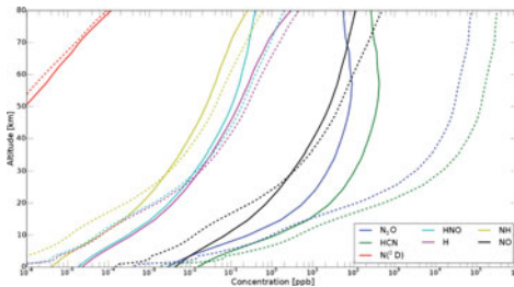
Figure 4. The radial profile of the steady state mixing ratios of atmospheric species forming as a result of photo-collisional processes in the early terrestrial atmosphere driven by an SEP event (Airapetian et al. 2016a).
