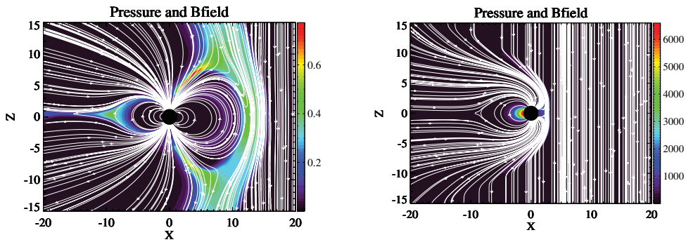
Figure 3. The initial (left panel) and final solution (right panel) for the magnetospheric structure driven by a SCME impact on the early Earth magnetosphere (Airapetian et al. 2015).
