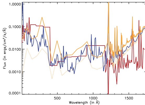
Figure 1. The SED in the XUV band for the solar X5.4 flare (blue) & the young Sun SED (orange) scaled to 1 AU and GJ 832 SED (red) scaled to 0.16 AU.
