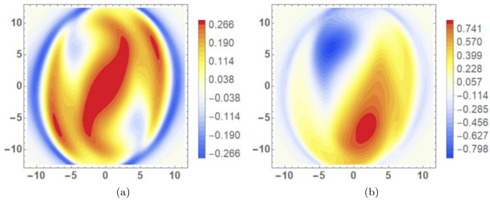
FIGURE 12. Vertical velocity distributions at t=28 . (a) The velocity density u_z(P_v(x,y))J at the moving photosphere line \rho=1 . (b) The difference between the varying photosphere velocity density u_z(P_v(x,y))J and the z=0 velocity density u_z(x,y) .
