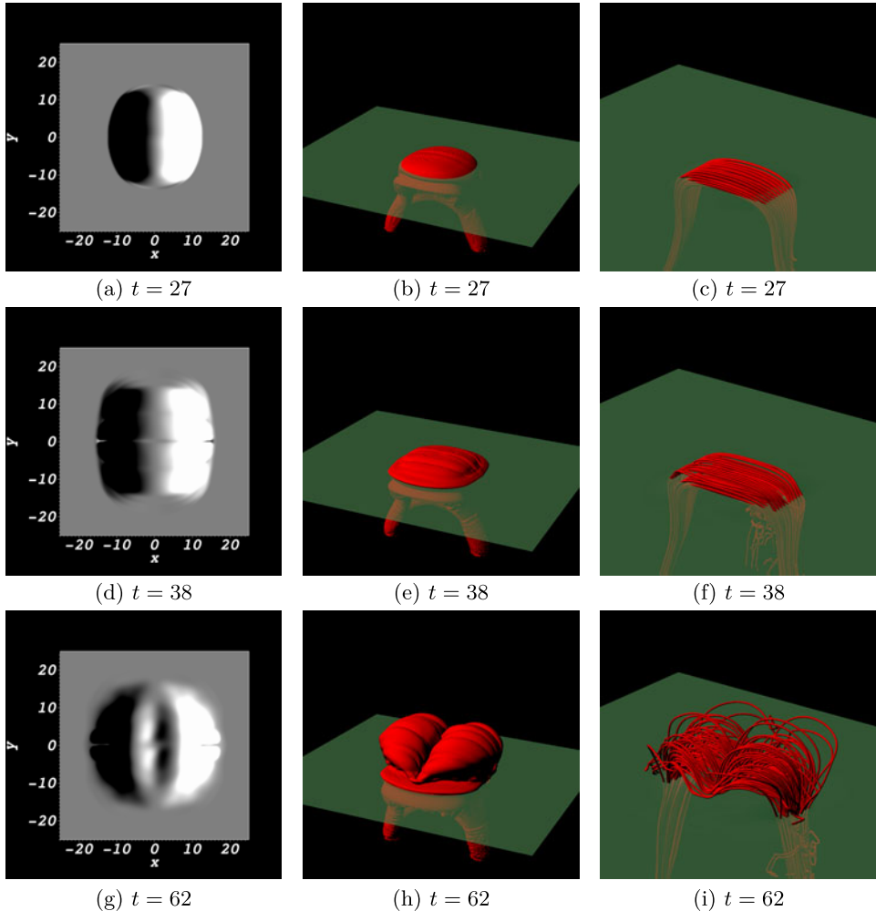
FIGURE 15. Illustrative distributions characterizing the emergence of a mixed helicity flux rope with n=2 twist pairs. (a,d,g) are magnetograms. (a) depicts ( t=27 ) a bipole structure associated with the initial emergence phase. In (d) ( t=38 ), this distribution has separated slightly and there also appear to be some weak thin horizontal structures appearing at the centre of the domain. In (g) ( t=62 ), these weak additional structures have developed into pairs of bipoles whose polarity oppose that of the larger initial bipole. (b,e,h) are current contours ( |j|=0.01 ) which indicate the field's expansion. Also indicated is the plane z=0 . (c,f,i) are representative field lines.
