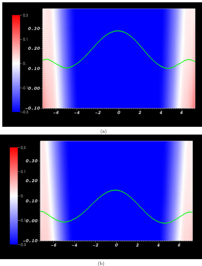
FIGURE 14. Magnified representations of a slice of the vector field in the plane orthogonal to the PIL at t=30 and t=31 , prior to and at the spike in the time series dL_v/dt shown in figure 11(d). Shown as a green curve is the intersection of the surface P_v and this plane. The background distribution is the out of plane component of the current density. (a) shows ( t=30 ) a magnification of the region of figure 13 which contains the curve \rho=1 . (b) shows ( t=31 ) the same distribution as in (a) but at the time of the spike. The \rho=1 curve has dropped vertically by a value of approximately 0.5.
