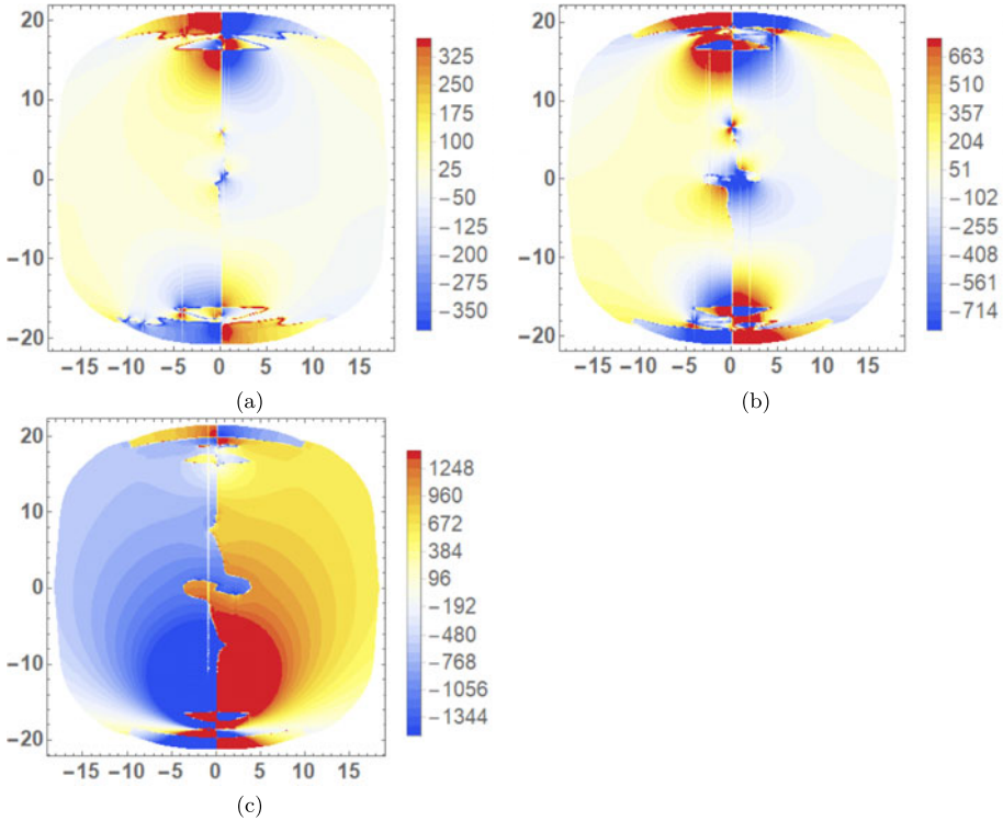
FIGURE 20. Distributions of the winding input density d\mathcal{L}_v/dt covering the period of the time series shown in figure 19(d) at which there is a strong spike in input. (a) At t=45 , before the spike. (b) At t=46 . (c) At t=47 at the spike's peak.
