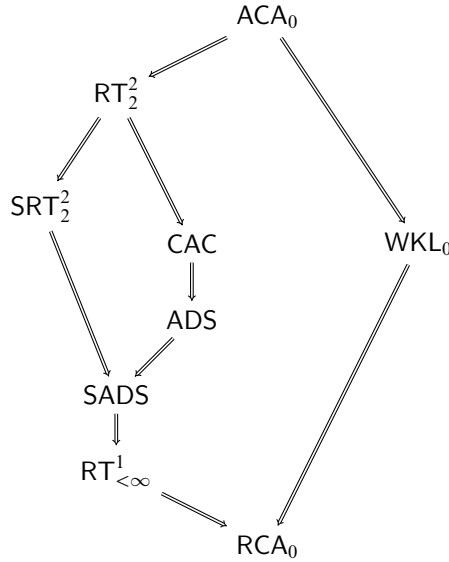
FIGURE 1. Selected principles and systems and their implications and non-implications over RCA_0 . An arrow indicates that the source principle/system implies the target principle/system over RCA_0 . No further arrows may be added, except those that may be inferred via transitivity. No arrows reverse. Proofs of these implications and separations may be found in [6, 8, 16, 17, 21, 22, 26, 29, 30].
