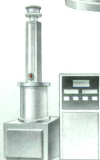
Crystal Growth
