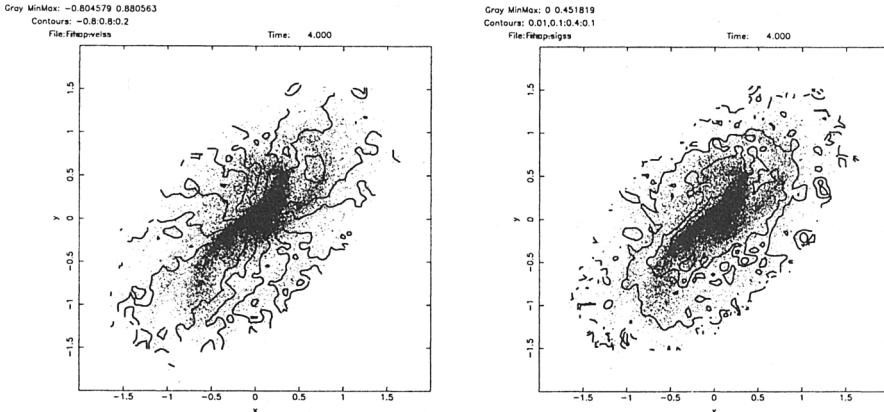
Figure 1. Example of graphics output from NEMO. On the left the mean velocity (1st intensity weighted moment), on the right the velocity dispersion (2nd velocity moment, corrected for mean streaming) in a bar unstable galactic disk.
