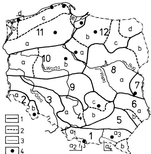
Fig 1. Subdivision of Poland into palaeoecological regions (Ralska-Jasiewiczowa, 1982). 1 \square —boundaries of main regions, 2 \square and 3 \square —boundaries of sub-regions, 4 \bullet —location of ref sites.
