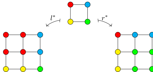
FIGURE 6 (colour online). For a 2-cube g: I_1^{\otimes 2} \rightarrow G of N_1 G , the map l^*: N_1 G \rightarrow N_2 G sends g to the 2-cube gl^{\otimes 2}: I_2^{\otimes 2} \rightarrow G of N_2 G , whereas r^*: N_1 G \rightarrow N_2 G sends g to the 2-cube gr^{\otimes 2}: I_2^{\otimes 2} \rightarrow G of N_2 G .
