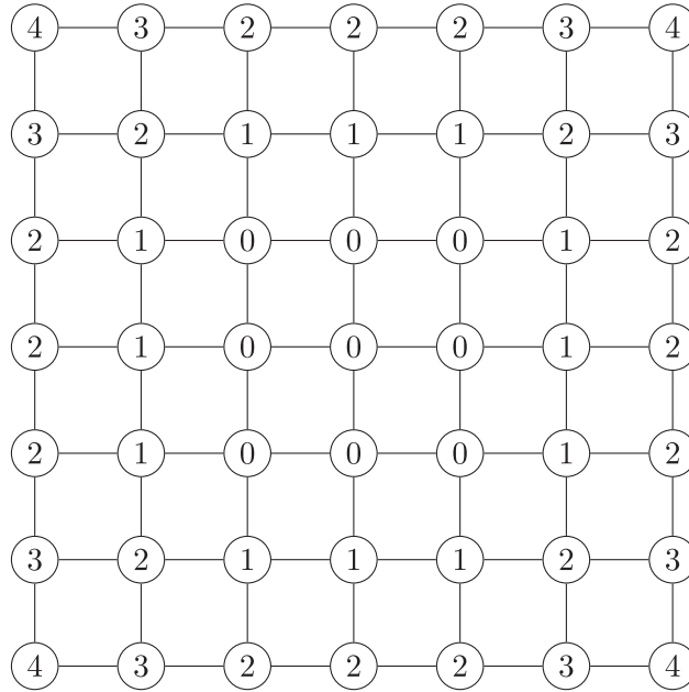
FIGURE 7. Vertices of I_6^{\otimes 2} labeled by their image under d: I_6^{\otimes 2} \rightarrow I_\infty .
