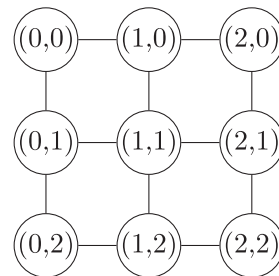
(d) The subgraph I_2^{\otimes 2} \otimes \{1\} under \lambda_{1,1}^2
