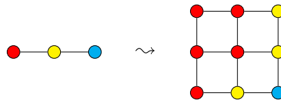
FIGURE 10 (colour online). The square g : I_2^{\otimes 2} \rightarrow G constructed from the path f : I_2 \rightarrow G .
