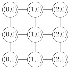
(c) The subgraph I_2^{\otimes 2} \otimes \{0\} under \lambda_{1,1}^2
