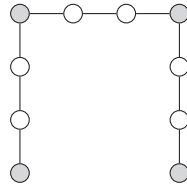
FIGURE 4. The graph |\square_{2,1}^2|_3 . The image of the embedding G_{3,0} \hookrightarrow |\square_{2,1}^2|_3 is shaded.
