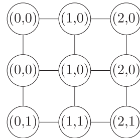
(b) The subgraph I_2^{\otimes 2} \otimes \{1\} under \lambda_{1,1}^2
