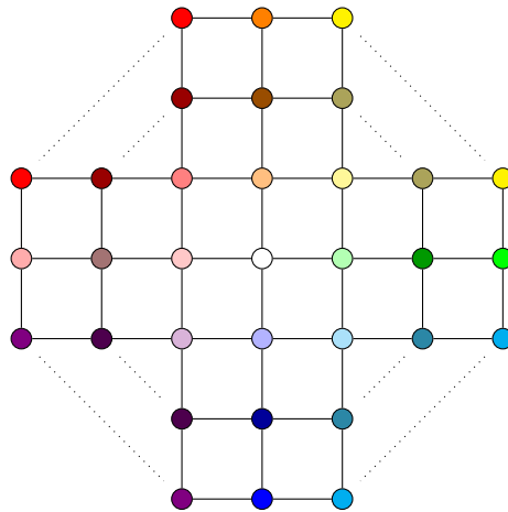
FIGURE 8 (colour online). The graph |\square_{3,1}^3|_2 as a net. Vertices connected by a dotted line are identical.
