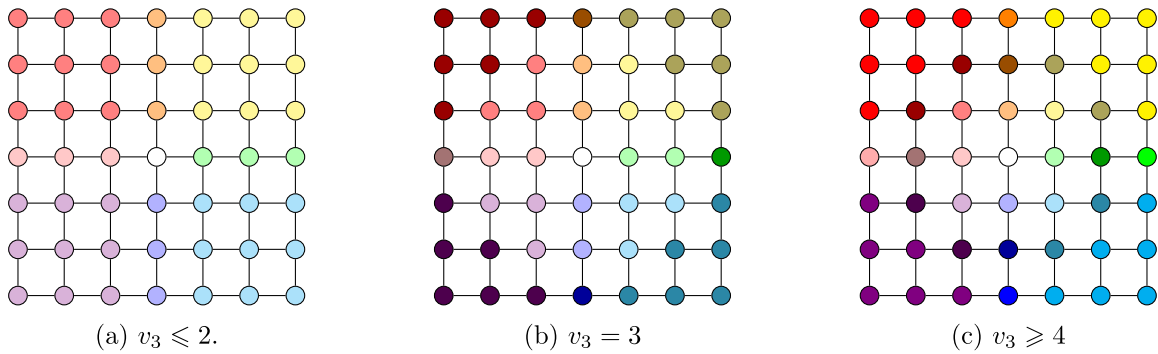
FIGURE 9 (colour online). The map \Phi: I_6^{\otimes 3} \rightarrow |\square_{3,1}^3|_2 split into cross-sections.
