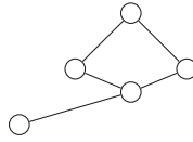
FIGURE 1. An example depiction of a graph.
