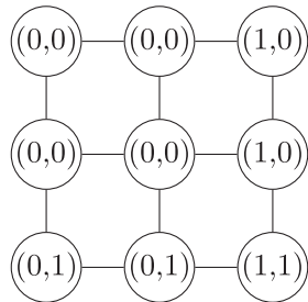
(a) The subgraph I_2^{\otimes 2} \otimes \{0\} under \lambda_{1,0}^2
