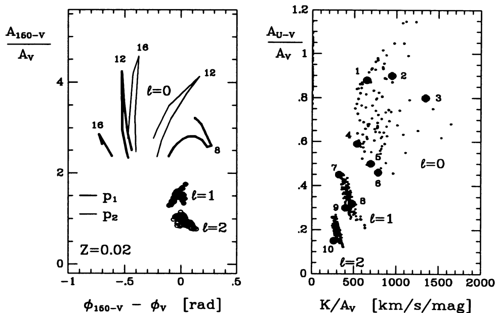
Fig. 1. (a) The ratio of color to light amplitudes is plotted against the phase difference for unstable modes in \beta Cephei models. For the case of radial pulsations, the plotted lines connect points, separately for p_1 (fundamental) and p_2 modes, corresponding to sequence of models, from the instability onset to the moment of hydrogen exhaustion in the core. The value of mass is given in M_{\odot} . Points plotted for the nonradial modes cover the same range of stellar models.
