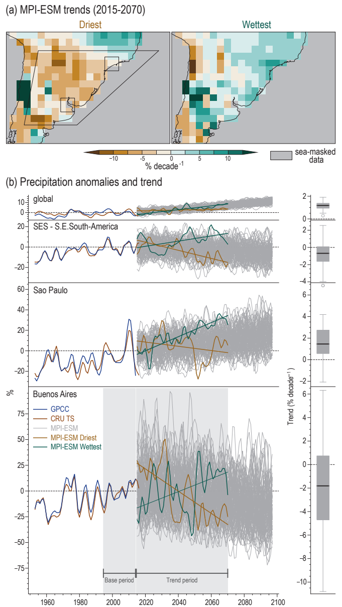
Figure 10.10 | Observed and projected changes in austral summer (December to February) mean precipitation in Global Precipitation Climatology Centre (GPCC), Climatic Research Unit Time Series (CRU TS) and 100 members of the Max Planck Institute for Meteorology Earth System Model (MPI-ESM). (a) 55-year trends (2015–2070) from the ensemble members with the lowest (left) and highest (right) trend (% per decade, baseline 1995–2014). (b) Time series (% , baseline 1995–2014) for different spatial scales (from top to bottom: global averages; South-Eastern South America; grid boxes close to São Paulo and Buenos Aires) with a five-point weighted running mean applied (a variant on the binomial filter with weights [1-3-4-3-1]). The brown (green) lines correspond to the ensemble member with weakest (strongest) 55-year trend and the grey lines to all remaining ensemble members. Box-and-whisker plots show the distribution of 55-year linear trends across all ensemble members, and follow the methodology used in Figure 10.6. Trends are estimated using ordinary least squares. Further details on data sources and processing are available in the chapter data table (Table 10.SM.11).
