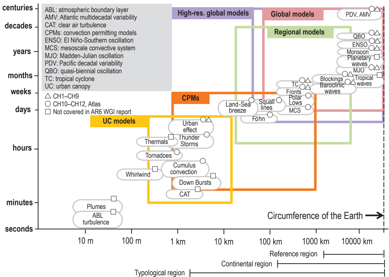
Figure 10.3 | Schematic diagram to display interacting spatial and temporal scales relevant to regional climate change information. Figure adapted from Orlandi (1975). The processes included in the different models and model components considered in Chapter 10 are indicated as a function of these scales. The various types of models (including global and regional climate models) for constructing regional climate information are assessed in Section 10.3.1 and Box 10.3.
