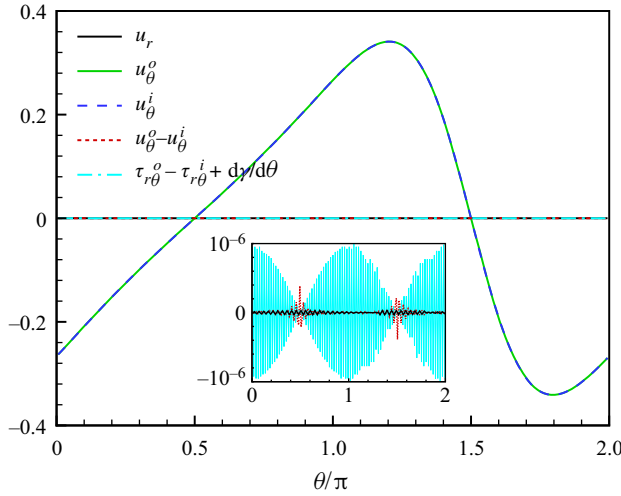
Figure 4. Velocity and force distributions on the external interface of a two-phase drop with \alpha = \pi , \beta^1 = \beta^2 = 1 and Pe = 6 .
