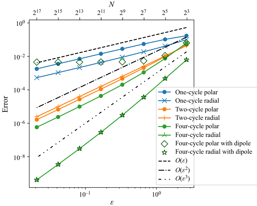
Figure 4. Convergence of the passive particle displacement with N repeated applications of the first-order control corresponding to \{h_1, h_2\} with control amplitude \varepsilon for a fixed target rotation by the angle \pi/6 about the origin.
