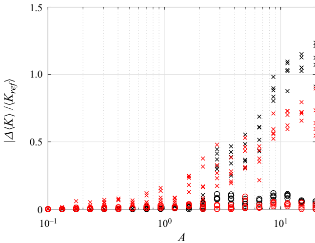
Figure 4. Relative error of the mean kinetic energy of the fluid induced by clusters for the two approximations, ( \times ): \langle K \rangle \approx \langle \mathbf{q}^T \mathbf{T}(\mathbf{q}) \mathbf{q} \rangle and ( \circ ): \langle K \rangle \approx \langle \boldsymbol{\xi}^T \mathbf{P}(\boldsymbol{\eta}) \boldsymbol{\xi} \rangle , against the excitation pressure amplitude with various polydispersities and values of B_0 . Black, (s_d, B_0) = (0.1, 0.5) ; red, (s_d, B_0) = (0.7, 5.0) .
