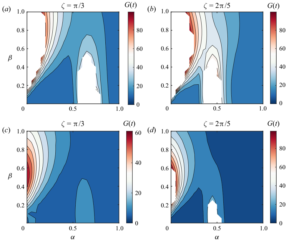
Figure 6. Contours of energy gain G(t) varying streamwise \alpha and spanwise \beta wavenumbers: (a,b) 21 km altitude; (c,d) 33 km altitude.
