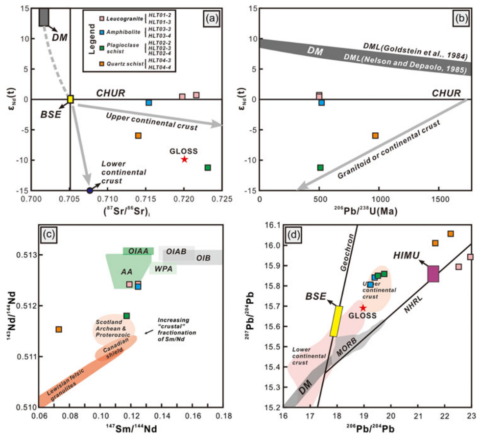
Figure 13. (a) (^{87}\text{Sr}/^{86}\text{Sr})_i versus \epsilon_{\text{Nd}}(t) diagram (after Winter and John, 2001; Wu et al. , 2003; Tang et al. , 2010a, 2010b), (b) ^{206}\text{Pb}/^{238}\text{U}(\text{Ma}) versus \epsilon_{\text{Nd}}(t) diagram (after Hu et al. , 2000; Winter and John, 2001), (c) ^{147}\text{Sm}/^{144}\text{Nd} versus ^{143}\text{Nd}/^{144}\text{Nd} diagram (after Goldstein et al. , 1984; Nelson and Depaolo, 1985), and (d) ^{207}\text{Pb}/^{204}\text{Pb} versus ^{206}\text{Pb}/^{204}\text{Pb} diagram (after Hart, 1984; White, 2003; Tang et al. , 2010a, 2010b) of the Hongliutian leucogranite and metamorphic rocks. Abbreviations: AA–Andean andesite, BSE–bulk silicate earth, CHUR–chondritic uniform reservoir, DM–depleted mantle, DML–depleted mantle line, Geochron for zero isochron line, GLOSS–global subducting sediment, HIMU–high U/Pb mantle, MORB–mid-ocean ridge basalt, NHRL–north hemisphere reference line, OIAA–oceanic island arc andesite, OIAB–oceanic island arc basalt, OIB–oceanic island basalt, and WPA–within-plate basalt. The data for marine sediments and global subducting sediment (GLOSS) are from Plank and Langmuir (1998) and Chauvel et al. (2008).
