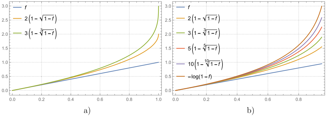
Figure 9. The values of \mathbf{E}v_j = \Phi_f(1/|I|) depending on f for equal stakes \alpha_j = 1/|I| . (a) |I| = 1, 2, 3 ; f \in [0, 1] . (b) |I| = 1, 2, 3, 5, 10, \infty ; f \in [0, .95] .
