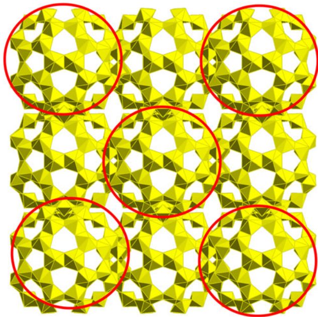
FIG. 1. One unit cell (a 5 37.884 Å, from the [100] direction) of the U 60 -bearing crystalline compound: Li 68 K 12 (OH) 20 [UO 2 (O 2 )(OH)] 60 (H 2 O) 310 with Li, K, and H 2 O omitted for clarity. Cluster molecules circled are in-plane with the page.
