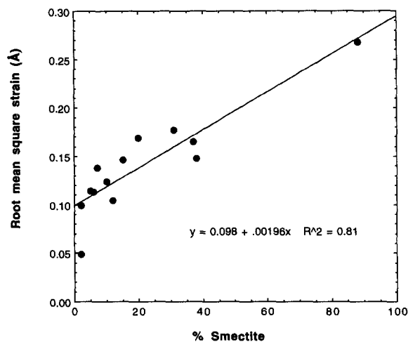
Figure 12. Relation between (\overline{\sigma_1^2})^{1/2} , measured from dehydrated I-S, and percent smectite layers, measured from glycol-solvated samples prior to dehydration.
