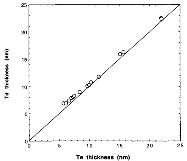
Figure 8. Mean thicknesses for the samples listed in Table 3 determined by extrapolation of Fourier coefficients ( \bar{T}_e ; see Figure 7A) compared with those determined from the distributions ( \bar{T}_d ; see Figure 7B) for the 001 reflection.
