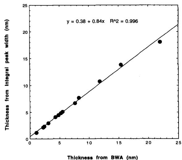
Figure 11. Relation between fundamental illite particle thicknesses calculated integral peak width thicknesses ( \bar{T}_i ) and expandability, and from BWA thickness ( \bar{T}_c ) and expandability using Equation [34].
