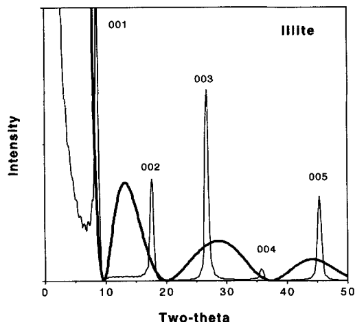
Figure 4. A NEWMOD ® -calculated illite XRD pattern (thin line) and its LpG^2 (thicker line).
