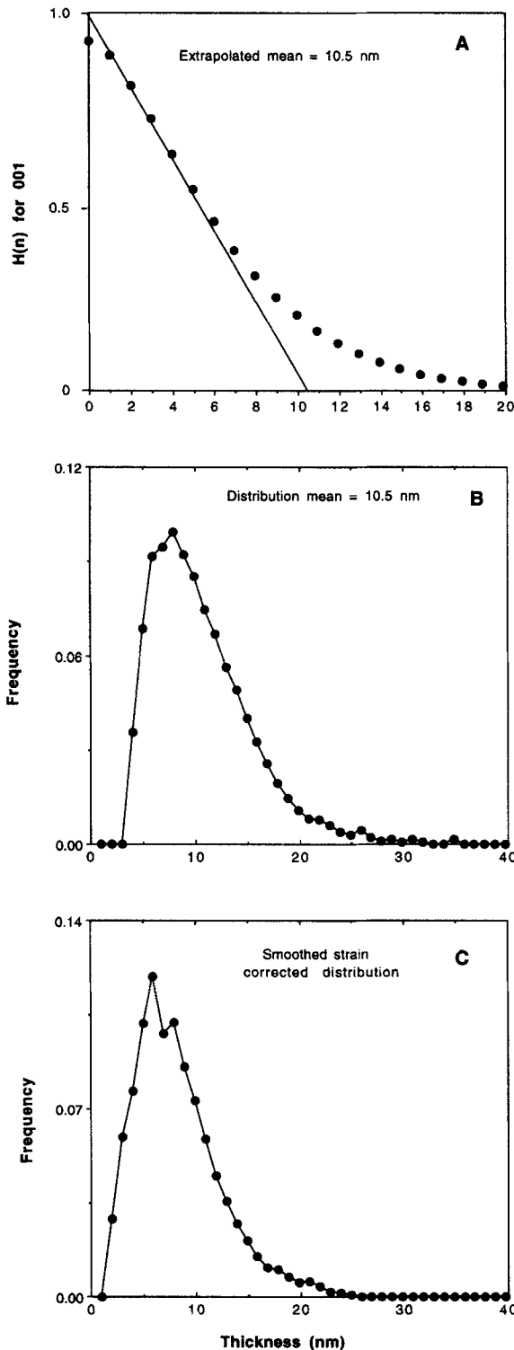
Figure 7. BWA analysis of K-saturated, dehydrated Zempleni sample. See Figure 5 for the XRD data. A = BWA method for determining the extrapolated mean ( \bar{T}_e ); B = crystallite thickness distribution calculated from the curve in A (no smoothing); C = crystallite thickness distribution calculated from Fourier coefficients that have been corrected for strain (smoothing power of 3).
