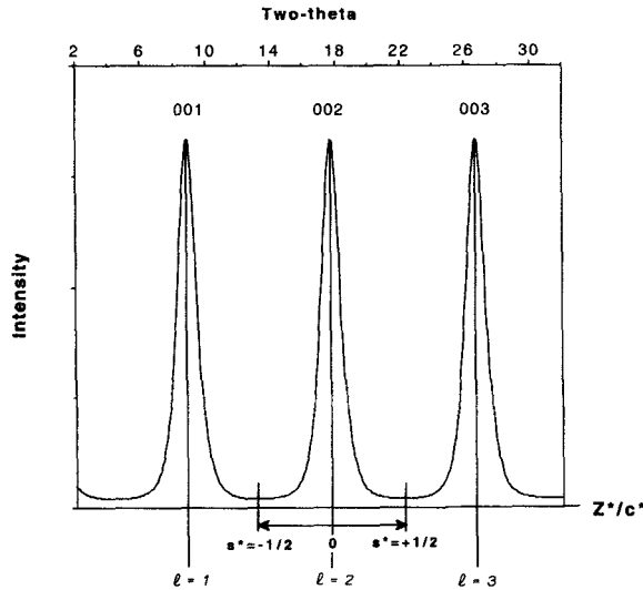
Figure 3. 00 l peaks of the interference function located along the Z^*/c^* axis. For the 002 peak, the origin is chosen at its maximum so that a new variable s^* may vary from -1/2 to +1/2 Z^*/c^* = l + s^* .
