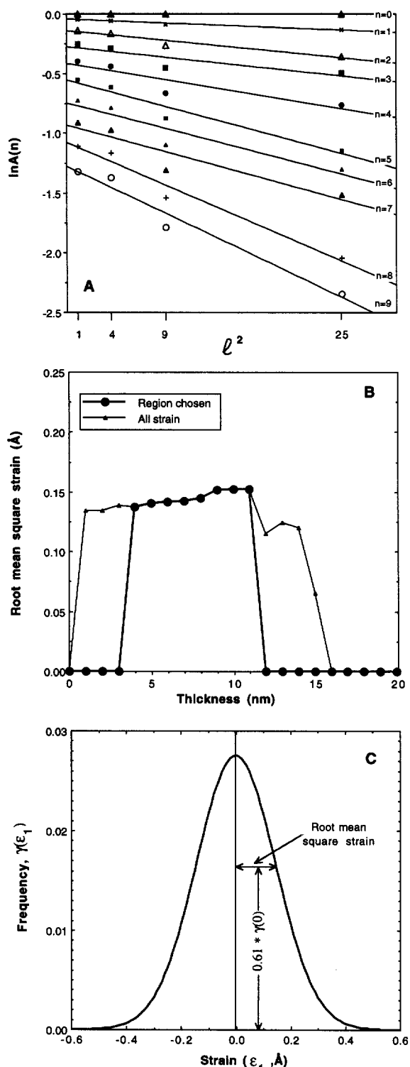
Figure 9. Strain determinations for the Zempleni sample made according to BWA theory. See Figures 5 and 7 for more information concerning this sample. A = plot used to determine the mean square of the strain ( \sigma_1^2 ) as a function of n ; B = the plateau in the root mean square strain data indicates that the strain ( \epsilon_1 ) has a Gaussian distribution; C = Gaussian strain ( \epsilon_1 , in Å) distribution ( \gamma(\epsilon_1) ; see Equation [24]) for this sample.
