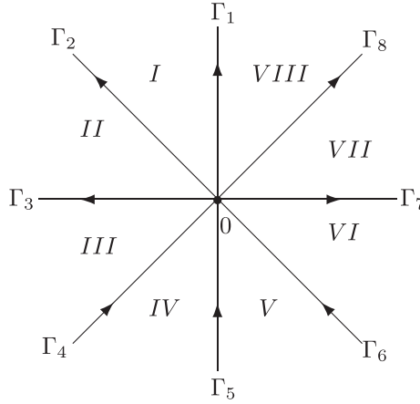
Figure B3. The jump contour \Sigma_{HG} for \Phi_{HG}(z) . The ray \Gamma_k is oriented from 0 to \infty , and forms an angle with \mathbb{R}^+ which is a multiple of \frac{\pi}{4} .
