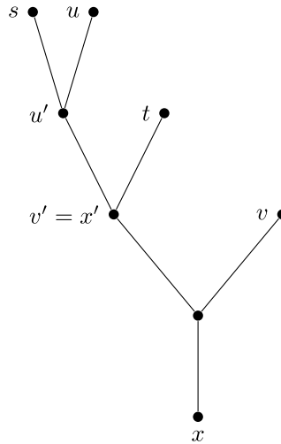
FIGURE 1. Possible positions of the closest point on the geodesic.
