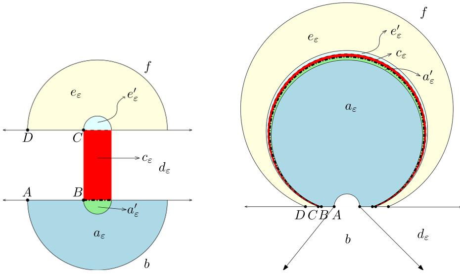
Figure 5. Reference and deformed configurations for the map u_\epsilon .
