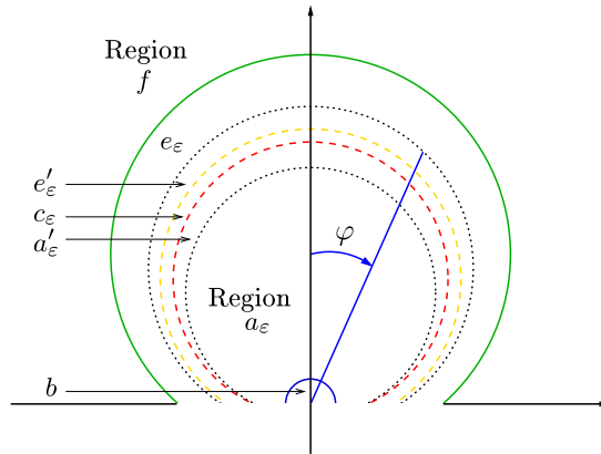
Figure 8. Schematic representation of the image of regions a_\varepsilon , a'_\varepsilon , c_\varepsilon , e'_\varepsilon and f after the deformation \mathbf{u}_\varepsilon . The parameter \varphi in the definition of \mathbf{u}_\varepsilon corresponds to the zenith angle in the deformed configuration.
