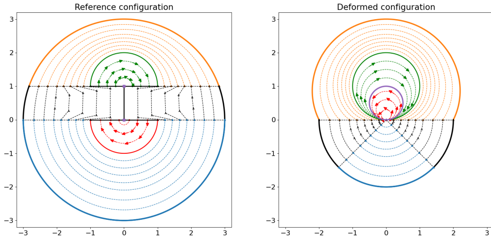
Figure 1. The 2D section of (a possible realization of) the Conti–De Lellis map [16]. The purple circle \{y_1^2 + y_2^2 + (y_3 - \frac{1}{2})^2 = \frac{1}{2^2}\} on the right is not attained as the image of any set of material points \mathbf{x} in \Omega = B(\mathbf{0}, 3) . It is, instead, new surface created by the map – that is, part of the boundary of the image of \Omega \setminus \{\mathbf{0}, \mathbf{0}'\} by \mathbf{u} , where \mathbf{0} = (0, 0, 0) and \mathbf{0}' = (0, 0, 1) are the only points where \mathbf{u} is singular.
