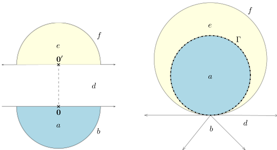
Figure 4. The map by Conti and De Lellis is defined differently in regions a to f . The reference and deformed configurations appear, respectively, on the left and on the right.
