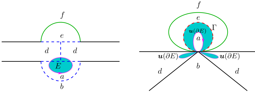
Figure 2. The Conti–De Lellis map [16] takes a portion of a given region E and sends it outside itself. The two closed curves in the right figure play a prominent role. One, on top, \Gamma , represented with a dashed circle, is a bubble created from two cavitation-like singularities. The other, \mathbf{u}(\partial E) , with self-intersections, enclosing three connected components, is represented with a dash-dotted line. Part of the coloured region on the right figure lies outside the dash-dotted loop, even though it consists of material points that were inside the dash-dotted curve in the reference configuration. Regions a – f are defined in Section 3; see also Figure 4.
