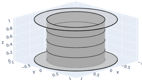
a) Reference configuration c_\epsilon
