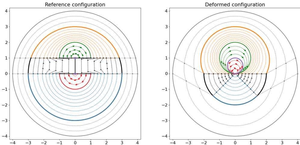
Figure 3. An extension of the Conti–De Lellis map [16] that satisfies the Dirichlet condition \mathbf{u}(\mathbf{x}) = \mathbf{x} on the boundary.
