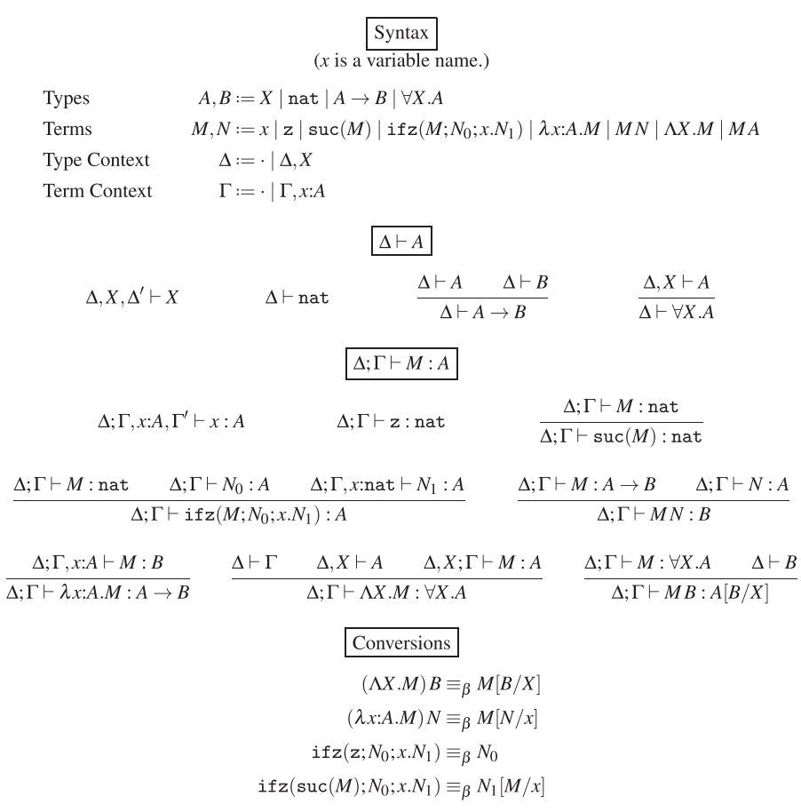
Fig. 2. Syntax, type rules, and conversion rules for System F.
