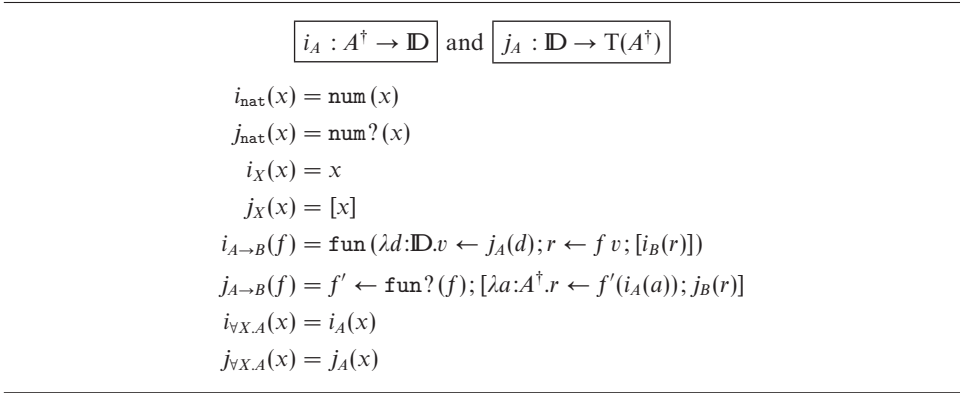
Fig. 5. Embeddings and projections
