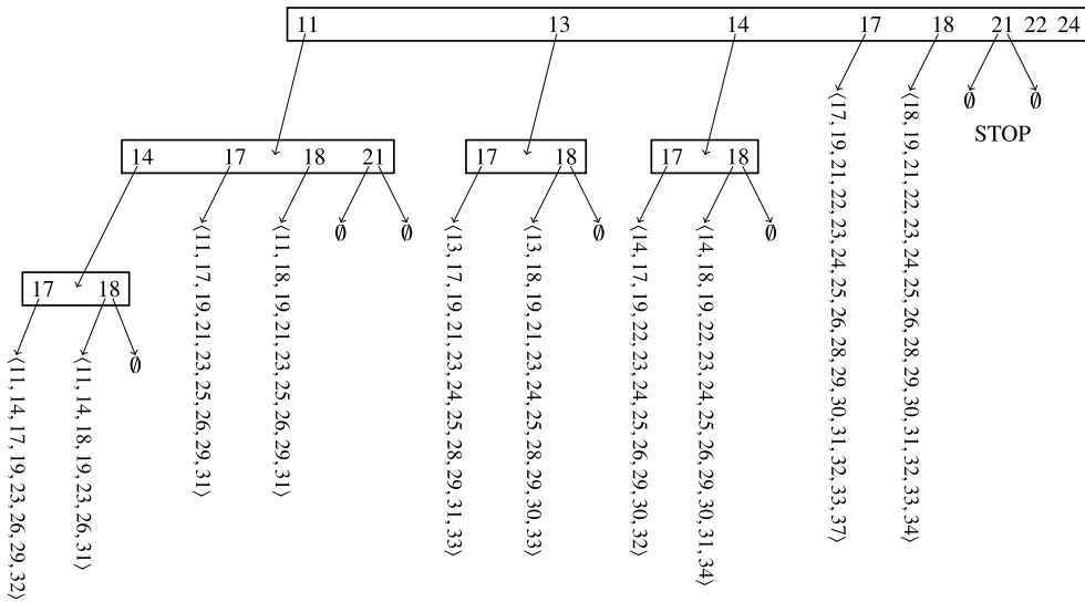
FIGURE 2. The numerical semigroups with pseudo-Frobenius numbers \{15, 20, 27, 35\} .
