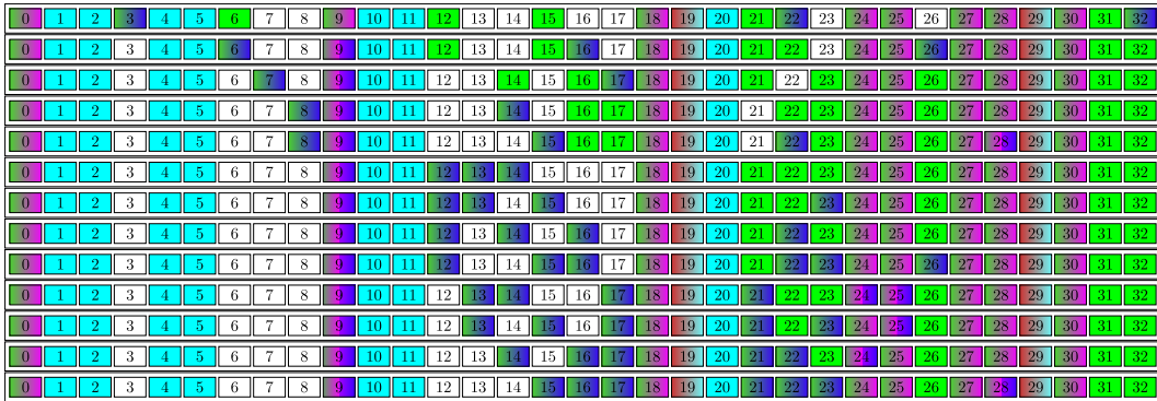
FIGURE 1. The numerical semigroups with pseudo-Frobenius numbers \{19, 29\} .
