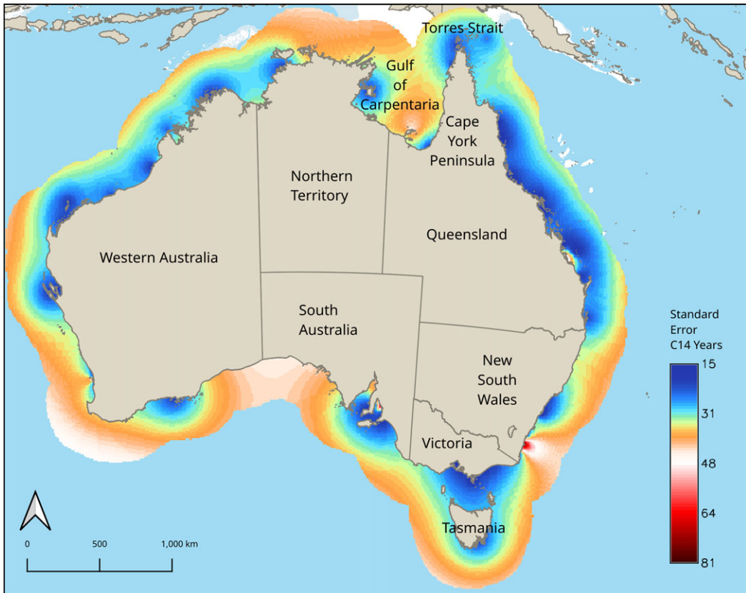
Figure 4 Overall standard error ( 14 C years) surface (combining both the standard errors of the original \Delta R measurements, and those of the interpolation process). Color scale shows range of \Delta R standard errors from small in blue with large in red. The kriging layer extends 300 km offshore from the closest mainland point.
