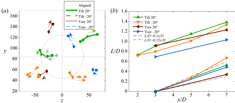
Figure 14. (a) Downstream development of vortex centre locations for different yaw and tilt angles. Increasing downstream location (data at x/D = 2, 3, 5, 7 ) is indicated by arrow. (b) Separation of vortex-core centres as a function of downstream location.
