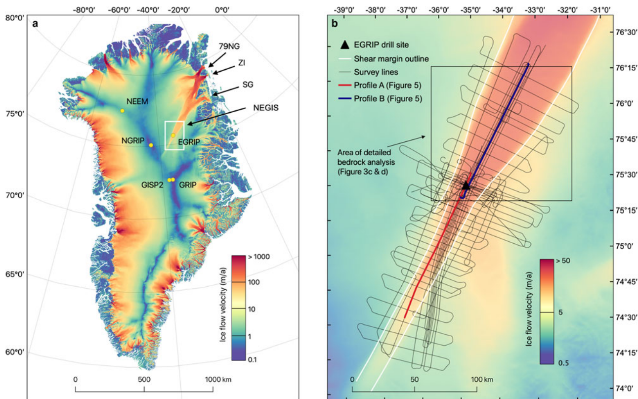
Fig. 1. (a) Surface velocity map of the Greenland ice sheet, highlighting the NEGIS and its marine-terminating outlets (79NG, Zachariae Isbrae (ZI) and Storstrømmen Glacier (SG)). The survey area (b) is marked with a white outline. (b) Ice flow velocity field of the survey area. The schematic outline of the shear margin was derived from Landsat images. Both maps are displayed in WGS 84/NSIDC Sea Ice Polar Stereographic North (EPSG:3413) and show velocity data of Joughin and others (2018).
