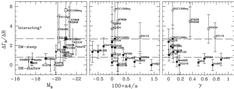
Figure 1. M/L gradients as a function of the intrinsic parameters. Dashed lines show a tentative separation between shallow and steep gradients and the interacting sample (see discussion in the text). In the left panel symbol dimensions are proportional to the outermost radii where M/L estimates are available.
