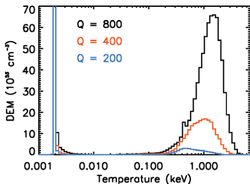
Figure 1. The time-averaged DEM from three 20 Msec RFHD simulations of \sigma Ori E, each differing only in the choice of opacity parameter \bar{Q} . Increasing \bar{Q} (bottom curve to top curve) leads to disproportionately stronger X-ray emission, and also hardens the spectrum.
