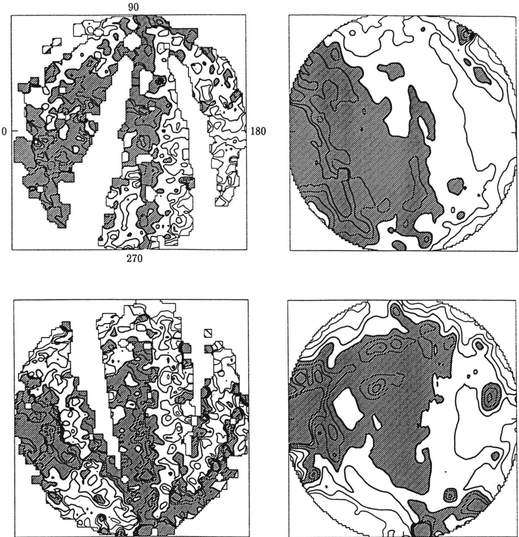
Figure 3. Contour and greyscale plot of the polar caps: top is North, bottom is South. Galactic poles are at the center of the maps, and radii are proportional to galactic latitudes from 90^\circ to 30^\circ or -90^\circ to -30^\circ . Polar angle is galactic longitude. On the left is the UV brightness and on the right is the far IR ( 100\ \mu\text{m} ) brightness. Both are cosecant law subtracted. Therefore the small-scale features are enhanced. The thickest contour (thickness 4) is the zero level. Contour thickness goes as the sequence 1234123. The increment for the contours is 3\ \text{nW m}^{-2}\ \text{sr}^{-1} in a 0.033\ \mu\text{m} band and 1\ \text{MJy/sr} resp. Grey parts correspond to positive excesses over the cosecant law, and white parts to negative excesses.
