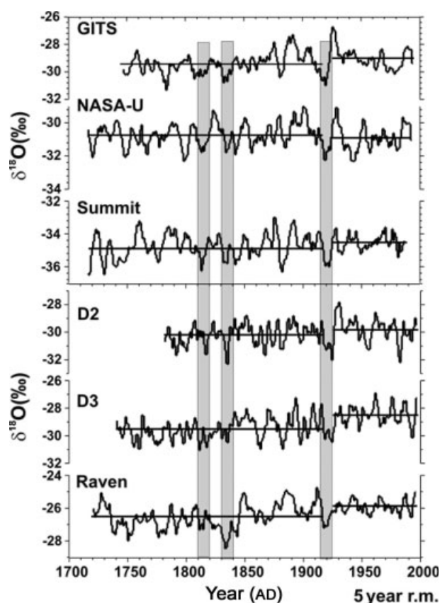
Fig. 2. The 5 year running mean of the annual \delta^{18}\text{O} histories from five new Greenland ice cores are shown along with the 1989 Site T record collected at the Summit (GISP2) site. Vertical shaded bars highlight specific time intervals discussed in the text. Horizontal bars in each record show the average \delta^{18}\text{O} value before and after the large cooling in 1917–19 that was followed by a rapid, widespread warming over much of the Arctic.
