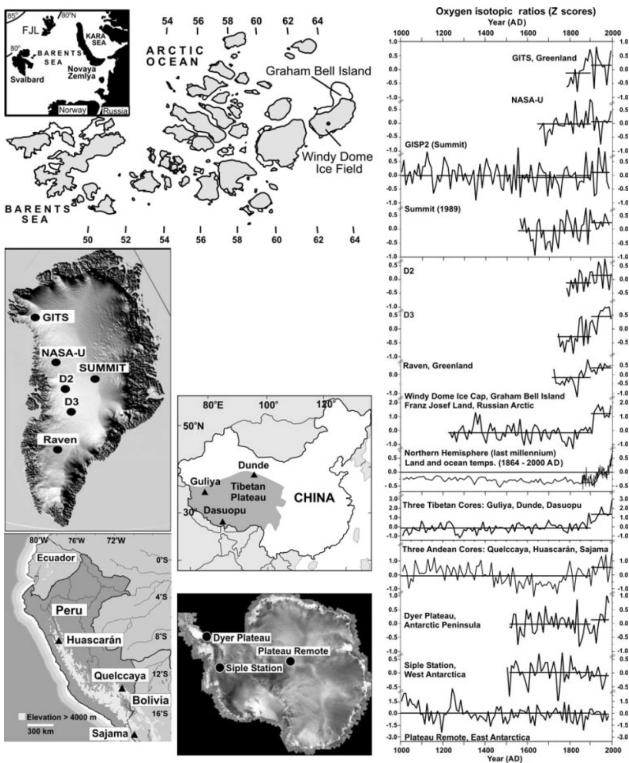
Fig. 1. Decadally averaged \delta^{18}\text{O} histories are shown from north to south (top to bottom). Horizontal bars in each record show the average \delta^{18}\text{O} values for the pre- and post-1900 time intervals. The 1000 year Northern Hemisphere reconstruction is from Mann and others (1999) and updated by Mann and Jones (2003). Superimposed is the observed near-surface temperature record (Jones and Moberg, 2003). Maps show locations for the cores.
