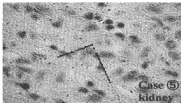
Fig. 3. \alpha -Particles travel straight even in tissues. The linear traces are those emitted by plutonium in the preserved kidney tissues of an A-bomb victim in Nagasaki (70 years ago) 11
