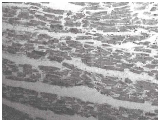
Fig. 3. \alpha -Particles travel straight even in tissues. The linear traces are those emitted by plutonium in the preserved kidney tissues of an A-bomb victim in Nagasaki (70 years ago) 11
