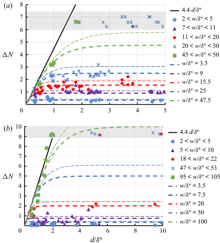
Figure 9. Variation of \Delta N with gap depth for different values of gap width for both (a) x_G = 450 \text{ mm} and (b) x_G = 127 \text{ mm} . Model predictions from (5.2), thick dash; model predictions from (5.3), thin dash; and experimental results, symbols.
