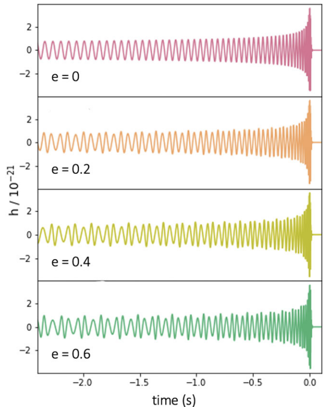
Figure 4. Example strain time series' of 30 M_{\odot} binary black hole mergers with four different eccentricities calculated at a reference frequency of 10 Hz. At relatively large eccentricity, modulations of the strain at periastron can resemble short-lived burst signals, especially at relatively large masses where only a couple of cycles may be present in the LIGO-Virgo-KAGRA observing band.
