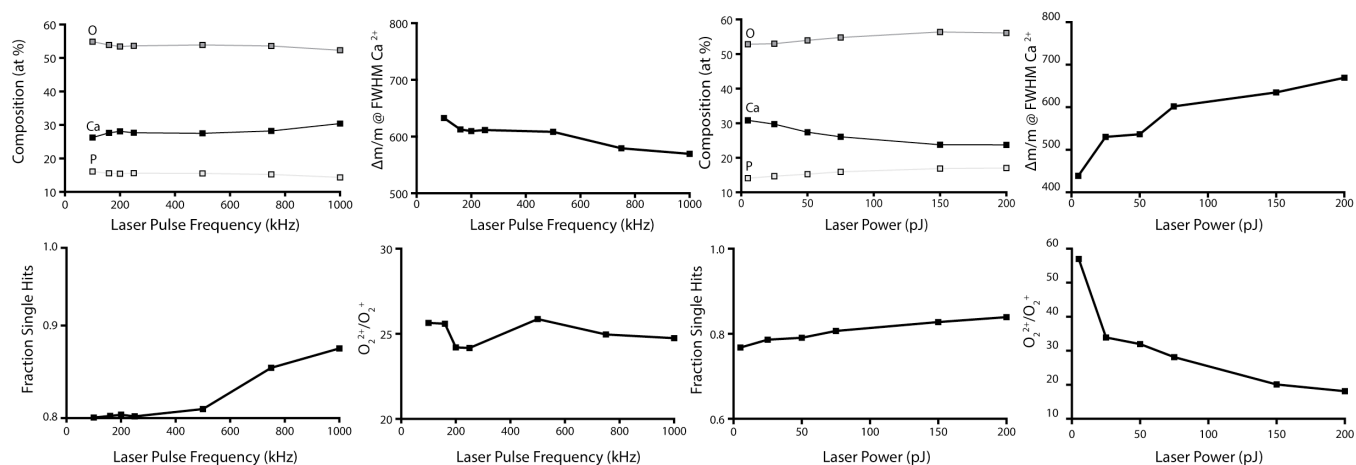
Figure 1. Optimization of stoichiometry (A, C), mass resolving power (B,D), single hit frequency (E,G), and charge state ratio (F,H) as a function of laser pulse frequency (A,B,E,F) and laser power (C,D,G,H).
