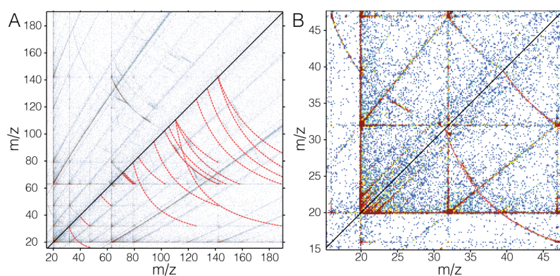
Figure 2. Double hit correlation histograms of a synthetic single crystal of hydroxylapatite. A. Correlation histogram with simulated decay tracks indicated below the diagonal (red arcs). B. Close up of (A), showing
