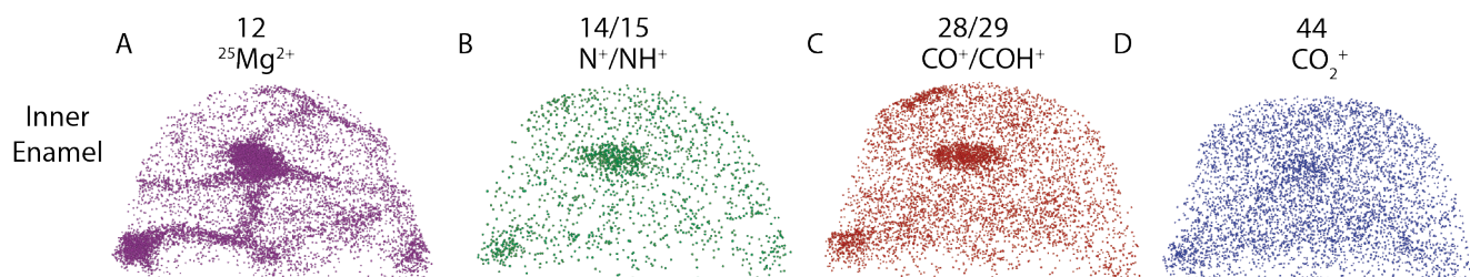
Figure 3. 3D Reconstructions of inner mouse enamel. A. Mg segregation at grain boundaries between hydroxylapatite nanowires. B. Nitrogen-containing ions in the intergranular precipitate. C,D. Carbon-containing ions originating from both organic and inorganic carbon.
