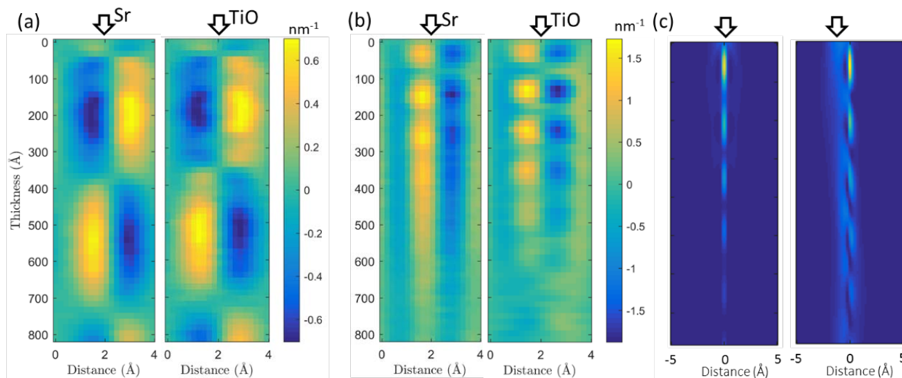
Figure 2. Simulated CoM images showing thickness oscillations in the probability current flow along Sr and TiO columns in [001] SrTiO 3 using a 10 mrad probe-forming semi-angle at 200 kV. CoM line profiles are for cut-off angles of (a) 4.3 mrad and (b) 120 mrad. (c) Real-space beam propagation for a probe directly on (left) and 0.8 Å away from (right) Ti column.
