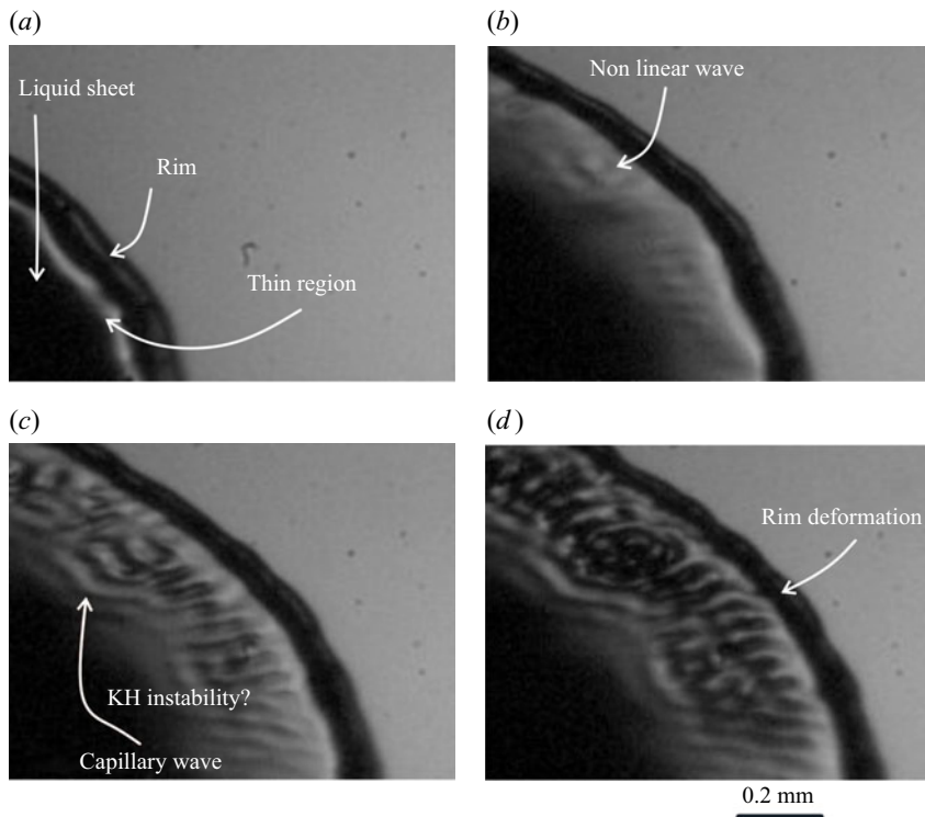
Figure 7. Formation of nonlinear Faraday waves and of the rim at the membrane-like region at the edge of the flattened droplet (a) rim formation, (b) initiation of nonlinear instability, (c) formation of capillary wave and (d) rim deformation due to radial acceleration and deceleration in the thinning regime just before the equatorial breakup.
