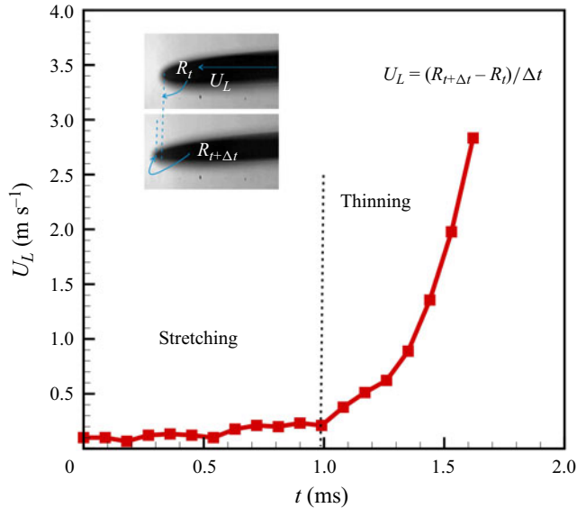
Figure 5. The radial velocity ( U_L ) of the radially expanding droplet before initiation of breakup. Note: the images are recorded at 11 000 fps with the camera focusing on the equatorial region of the droplet. Here, U_L is calculated for the 1.62 ms before initiation of breakup which covers both the stretching as well as the thinning regime ( We between 1.56 and 1.9).
