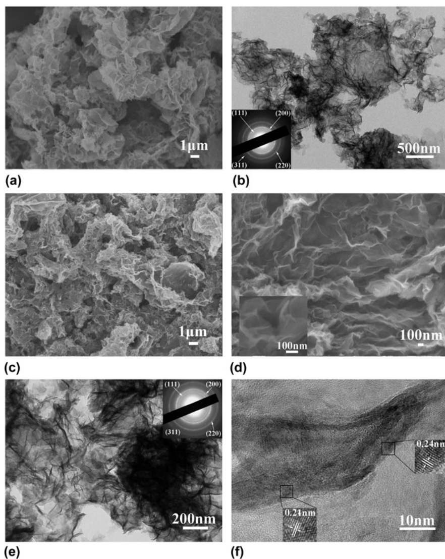
FIG. 12. (a) SEM image and (b) TEM image of the pure \text{NiCoO}_2 and the inset is the corresponding SAED pattern; (c) and (d) SEM images of the \text{NiCoO}_2/\text{rGO}/\text{NiCoO}_2 composite; (e) TEM image and (f) HRTEM of the \text{NiCoO}_2/\text{rGO}/\text{NiCoO}_2 composite. The inset in e is the corresponding SAED pattern.
