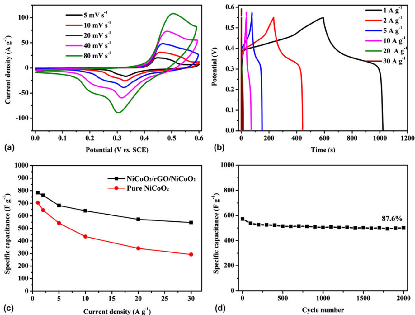
FIG. 13. (a) CV curves and (b) galvanostatic charge/discharge profiles of the NiCoO 2 /rGO/NiCoO 2 electrode in three electrode configurations; (c) specific capacitance of the pure NiCoO 2 electrode and NiCoO 2 /rGO/NiCoO 2 electrode at various current densities; (d) cycling performance of the NiCoO 2 /rGO/NiCoO 2 electrode at a current density of 20 A/g.
