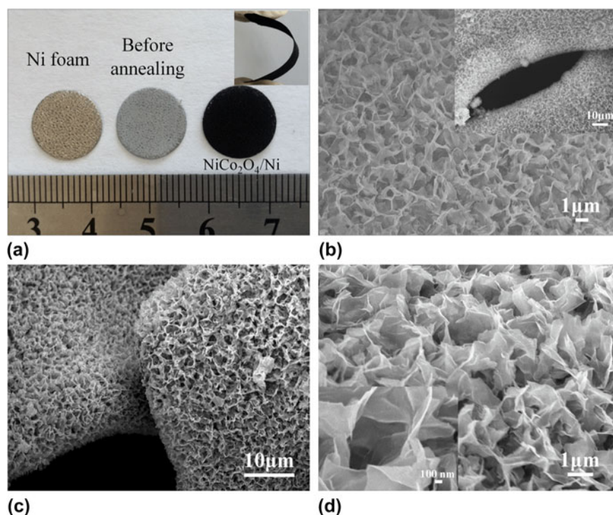
FIG. 1. (a) Pictures of the Ni foam before and after the annealing of \text{NiCo}_2\text{O}_4/\text{Ni} , and the inset is the photograph of a flexible \text{NiCo}_2\text{O}_4/\text{Ni} before punching; (b) SEM image of the Ni foam before the annealing of \text{NiCo}_2\text{O}_4/\text{Ni} ; (c) low-magnification SEM image of \text{NiCo}_2\text{O}_4/\text{Ni} after annealing; (d) high-magnification SEM image of \text{NiCo}_2\text{O}_4/\text{Ni} after annealing and the inset is partial enlarged detail.
