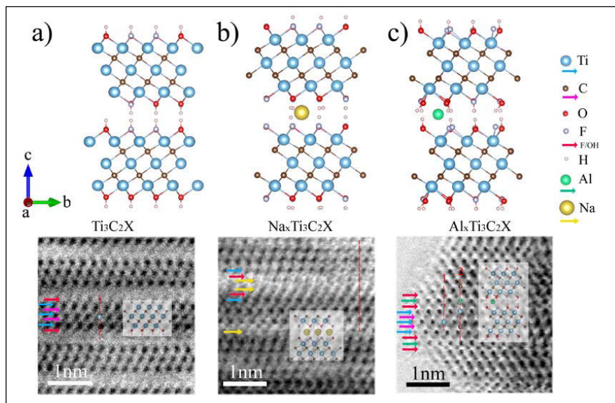
Figure 1. Optimized geometries of Ti_3C_2X (a), Na_xTi_3C_2X (b), Al_xTi_3C_2X (c) from cross-sectional view and corresponding ABF images.
