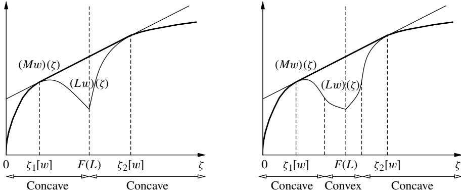
FIGURE 1: Two possible forms of (Lw)(\cdot) and their smallest nonnegative concave majorants (Mw)(\cdot) .
