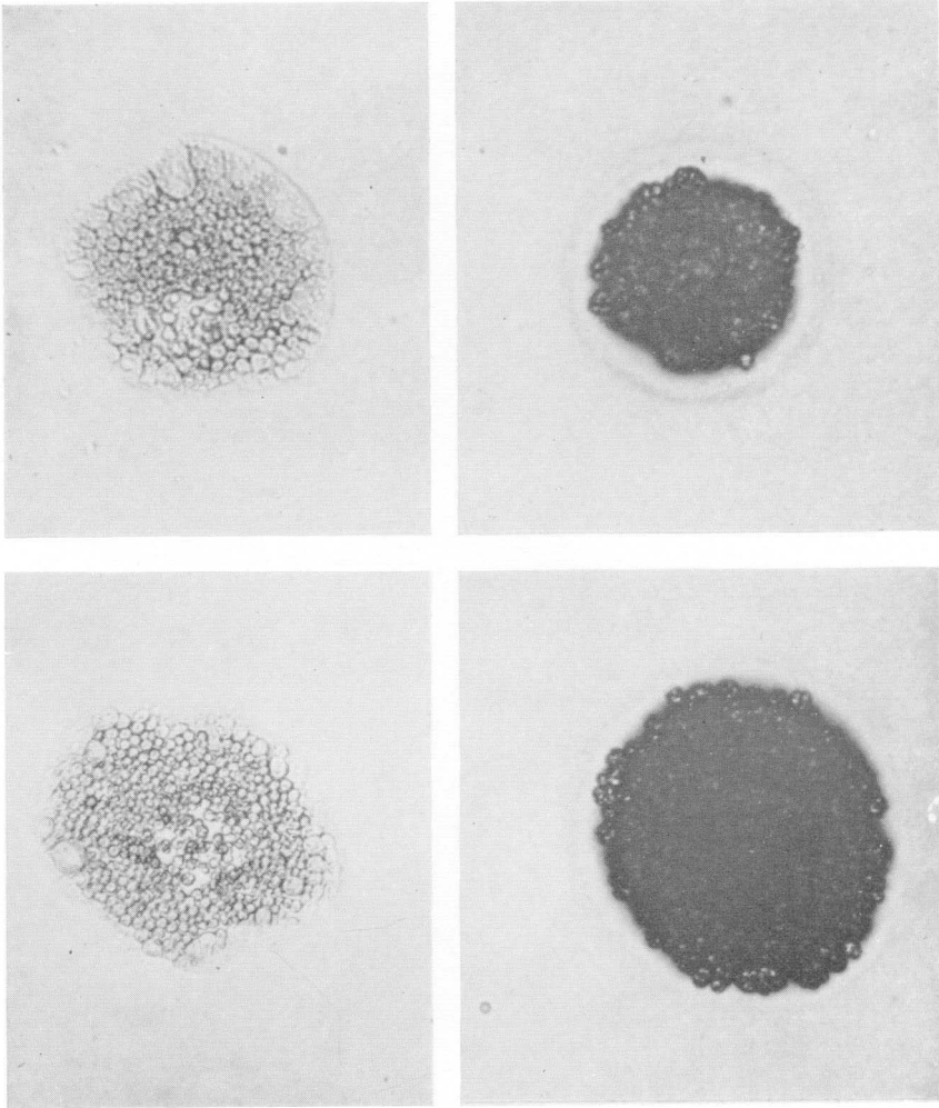
A tetrad derived from a CW2 × WT cross showing 2:2 segregation for the CW and WT phenotypes.
