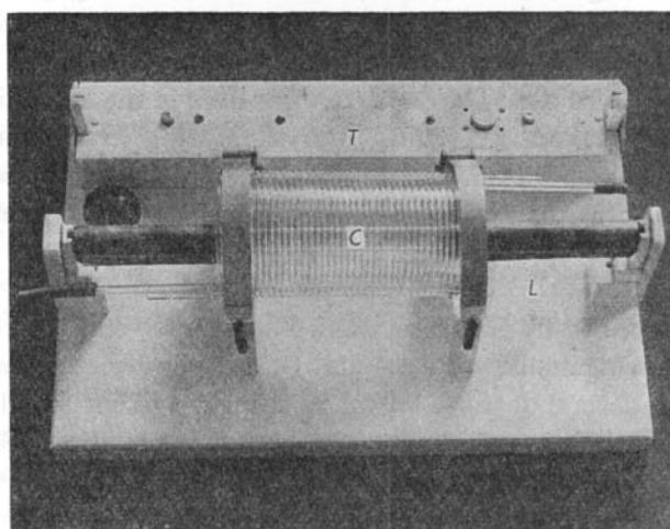
Fig. 1. Continuous flow irradiator of clear quartz tubing. C , coil; L , lamp with metal masks in position; T , channel for testing lamp prior to use. The apparatus is shielded by a metal cover while in use.
