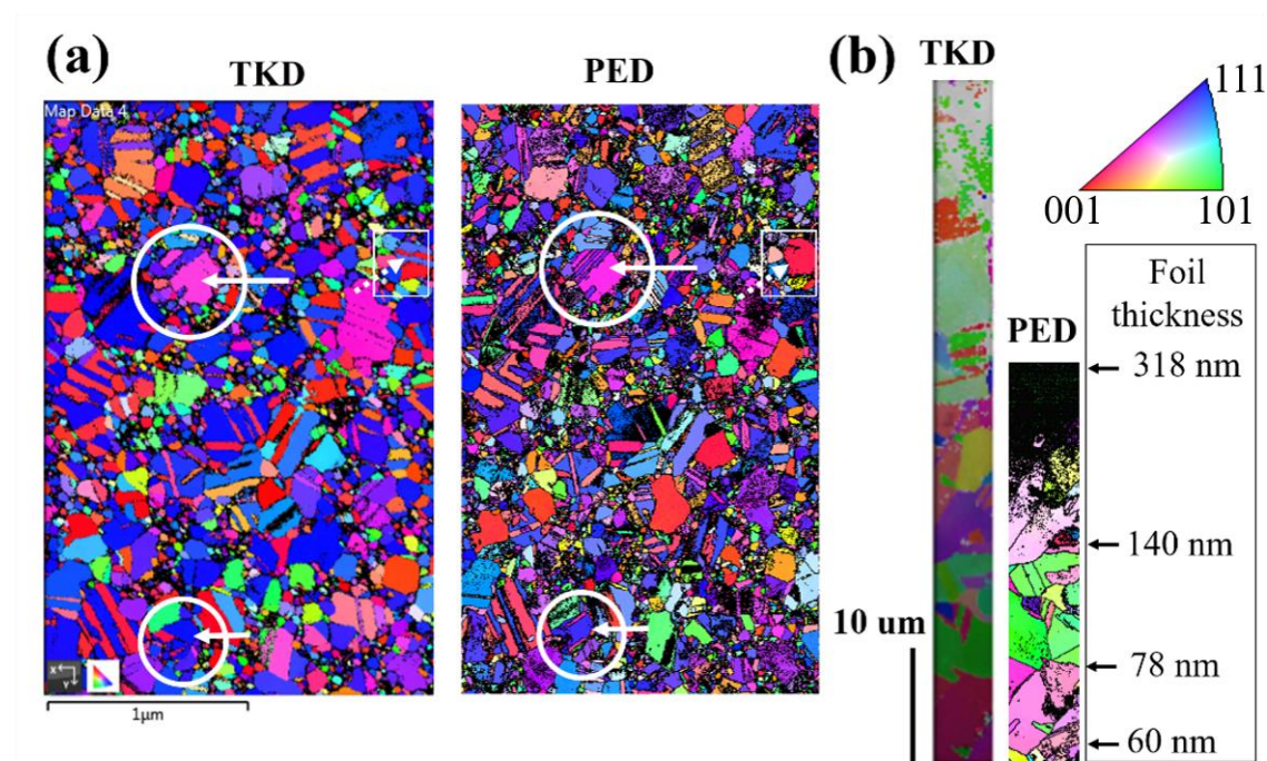
Figure 1. (a) TKD and PED map of a nanocrystalline Cu foil. The circled and solid arrows identify regions where PED revealed a higher spatial detection of twins whereas the boxed and dashed arrow identifies a region where TKD identified a twin that is absent in the PED scan. Each scan was done at a 5 nm step size. (b) A profile of collected Cu grains from the same region between TKD and PED as a function of foil thickness (measured by EELS). Note the further detection of the patterns for the TKD for thicker foils.
