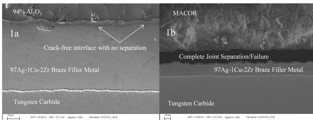
Figure 1. Different results were obtained using different ceramic substrates. Acceptable Joint (1a) made by brazing alumina ceramic to tungsten carbide with 97Ag-1Cu-2Zr active brazing filler metal. Total joint failure (1b) observed when brazing MACOR ® to tungsten carbide using the same brazing filler metal, 97Ag-1Cu-2Zr.
