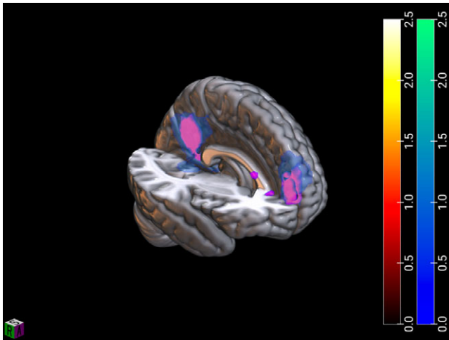
Figure 1. Cross-sectional analyses of the brain regions engaged in ABM vs. Object recall in both groups at follow-up (T2, depicted in blue-green) revealed a network consisting of the ventromedial prefrontal cortex (vmPFC), retrosplenial cortex (rSC), posterior cingulate cortex (pCC), MTG (middle temporal cortex) as well as hippocampus. This network showed a substantial overlap (depicted in pink) with the network that we found to be active at T1 (depicted in red-yellow).
