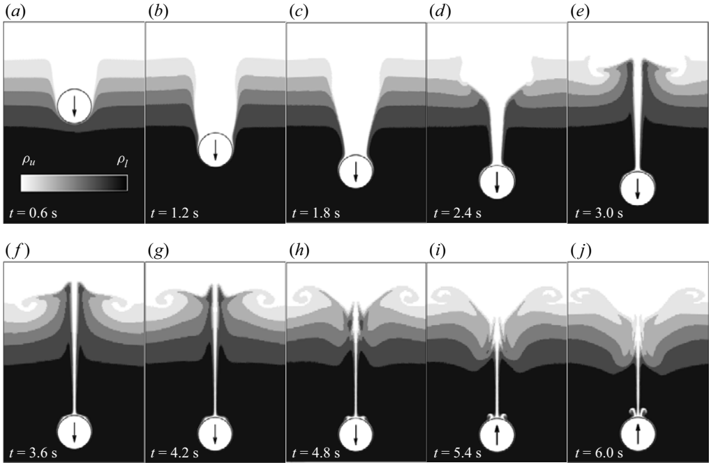
Figure 15. Simulated density field, using the same physical parameters as the experiment depicted in figure 12, presented for comparison with figure 14.
