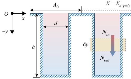
Figure 3. Schematic of the rectangular roughness.
