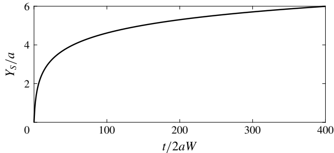
FIGURE 7. The temporal development of the scaled width Y_S/a of the constant (in x ) width current in the neighbourhood of the source forced by the uniform discharge (4.1) as a function of the scaled time t/2aW , as given by the formula (4.3). For positive PVa and negative PVa with a \geq 1 , the expansion terminates in the formation of a steady hydraulic solution. For negative PVa with a < 1 , so KW flow dominates, the expansion continues indefinitely but slows dramatically at larger times.
