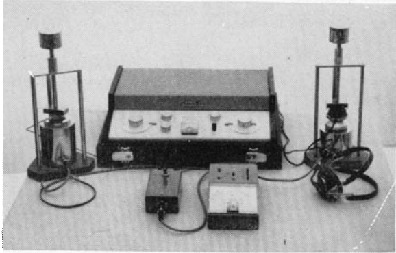
Kamplex set-up for Audiometer Calibration
