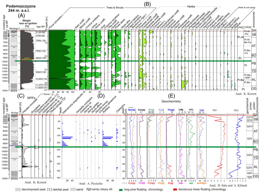
Figure 3 A—Litostratigraphic sequence of the Podemsczyzna fen with loss on ignition curve (A) and with modeled age scale (on the basis of age-depth model). The position of subfossil trees in the deposits was reconstructed on the basis of modeled age. B—pollen percentage diagram of terrestrial plants (selected taxa), with LPAZ and chronozones (det. by K. Korzeń); C—percentage diagram of aquatic, mire plants, and non-pollen palynomorphs (NPPs) (det. by K. Korzeń), D—percentage diagram of Rotifera and Cladocera (det. by A. Pocięcha), E—geochemistry of peatland deposits (det. by D. Sala and A. Klimek). PCA1 and PCA2 calculated by K. Bucek.
