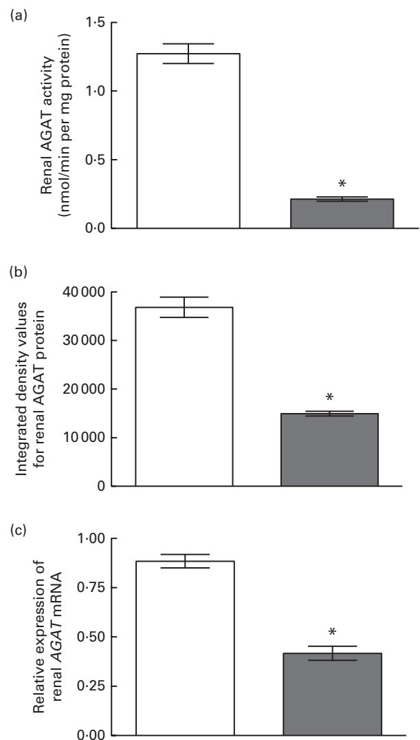
Fig. 2. Effect of dietary creatine on renal arginine:glycine amidinotransferase (AGAT). (a) Enzyme activity, (b) integrated density values from AGAT Western blotting and (c) relative expression of AGAT mRNA in the kidney. Creatine-free diet-fed group (□) and creatine-supplemented diet-fed group (■). Data for mRNA target genes were normalised to 18S ribosomal RNA. Values are means ( n 5), with their standard errors represented by vertical bars. *Mean values were significantly different between the dietary treatment groups ( P < 0.05).
