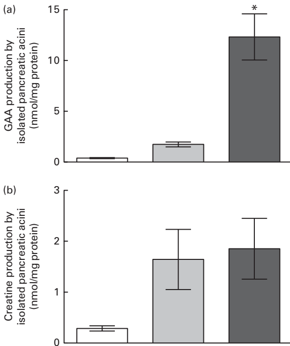
Fig. 3. Guanidinoacetate (GAA) and creatine production by acini isolated from the rat pancreas. (a) GAA production and (b) creatine production at time zero (□), after 40 min of incubation with 0.2 mM-glycine and 0.2 mM-arginine (▤), and after 40 min of incubation with 2 mM-glycine and 2 mM-arginine (▥). Values are means ( n 5), with their standard errors represented by vertical bars. *Mean values was significantly different between the 40 min incubations ( P < 0.05 ).
